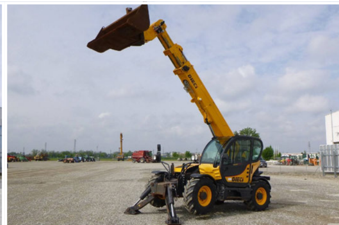
2015 DIECI RUNNER 40.13
