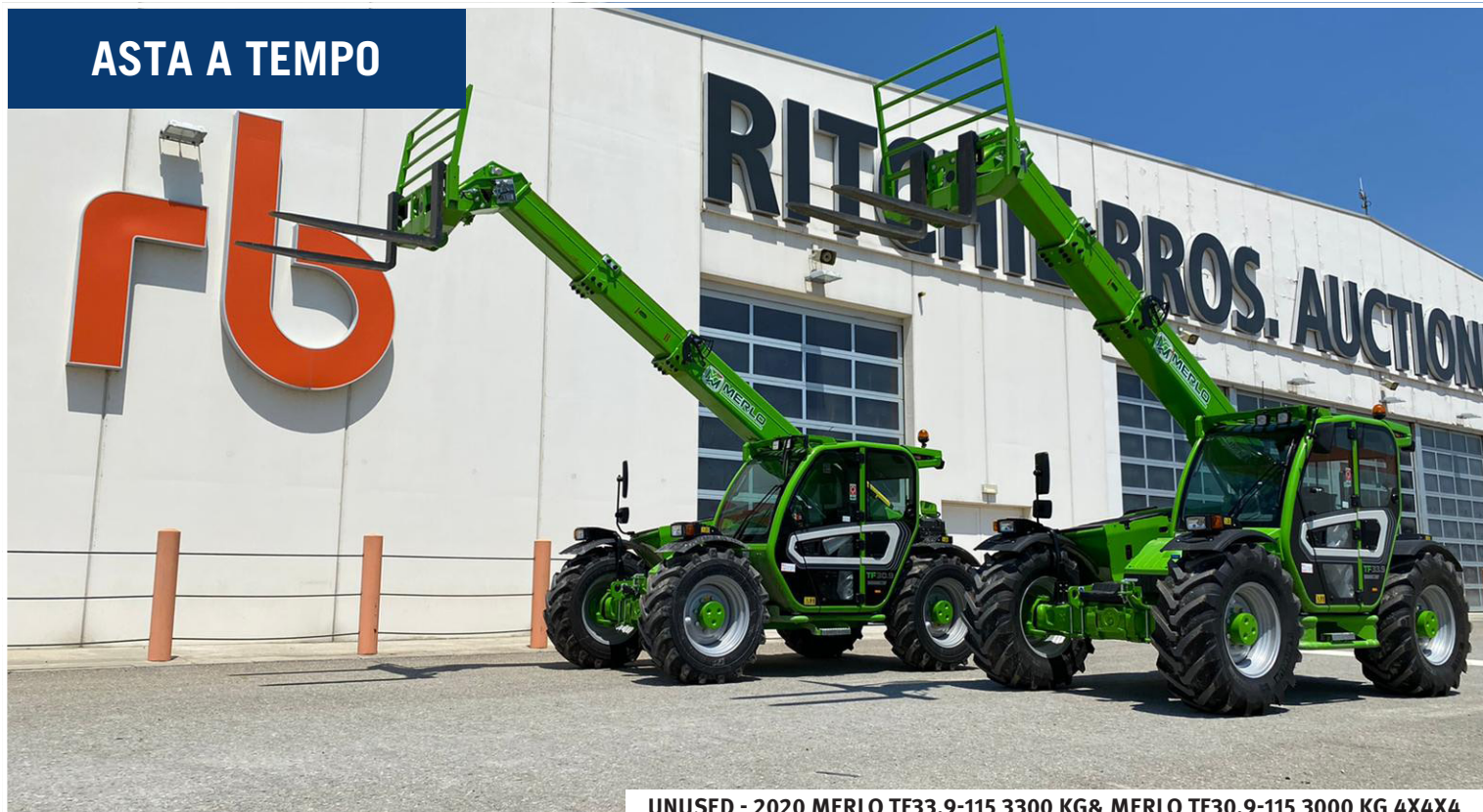
UNUSED - 2020 MERLO TF33.9-115 3300 KG& MERLO TF30.9-115 3000 KG 4X4X4
